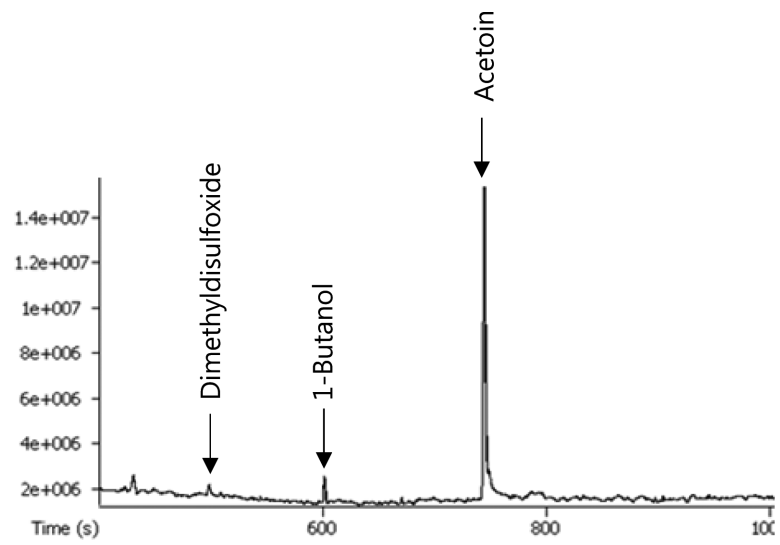
Supplementary Fig. 1. GC-MS total ion chromatogram of the volatile compounds produced by Bacillus velezensis G341.
