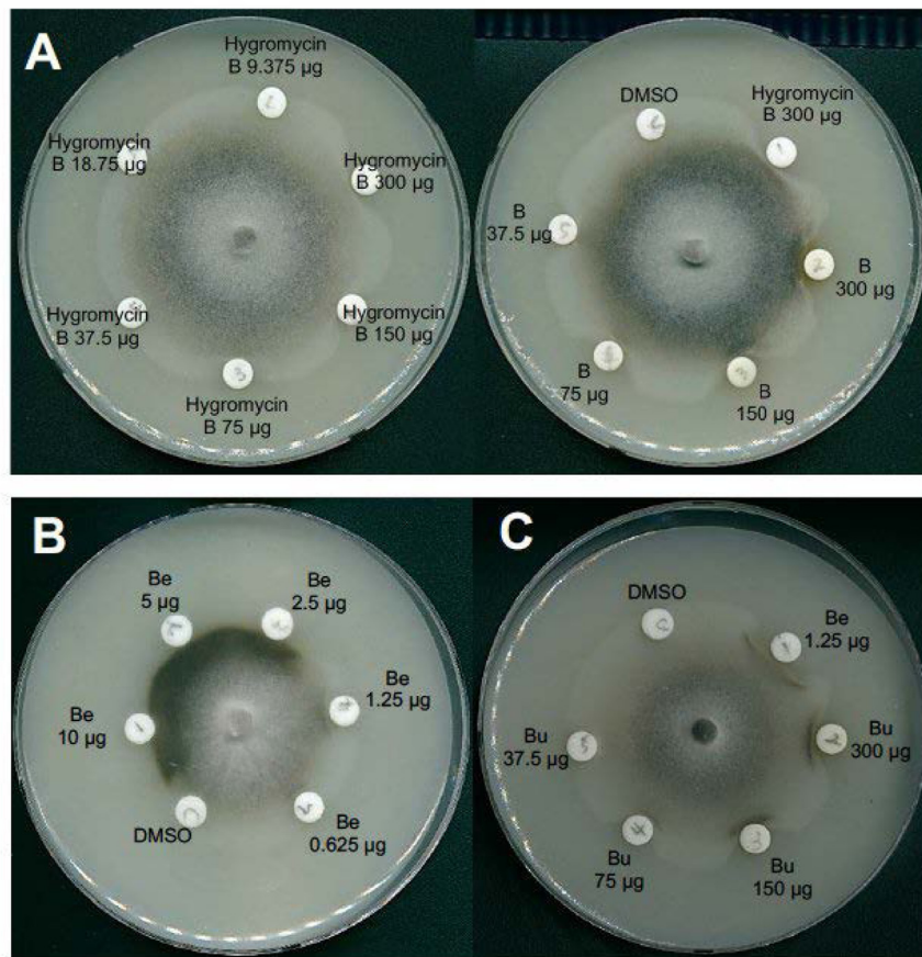
Supplementary Fig. 1. (A) Comparison of antifungal activity of Actinostemma lobatum butanol extract (plate on the right) with varying concentration of hygromycin B (plate on the left). (B) Inhibition effect of benomyl (Be) at various concentrations against Magnaporthe oryzae KJ201 mycelial growth. (C) The inhibitory effect of butanol extracts (Bu) at various concentrations against mycelial growth of M. oryzae .
