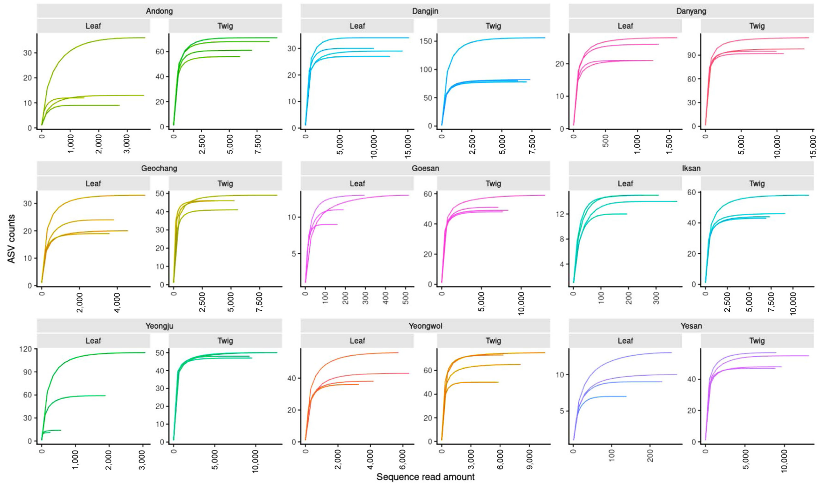
Supplementary Fig. 2. The rarefaction curve illustrates the relationship between read amount and amplicon sequence variant (ASV) counts, with the horizontal axis representing the former and the vertical axis the latter. As ASV counts increase, the lines on the graph become more parallel with the horizontal axis, indicating a decreasing likelihood of discovering new ASVs. Thus, the sample is indicative of the microbiota well.
