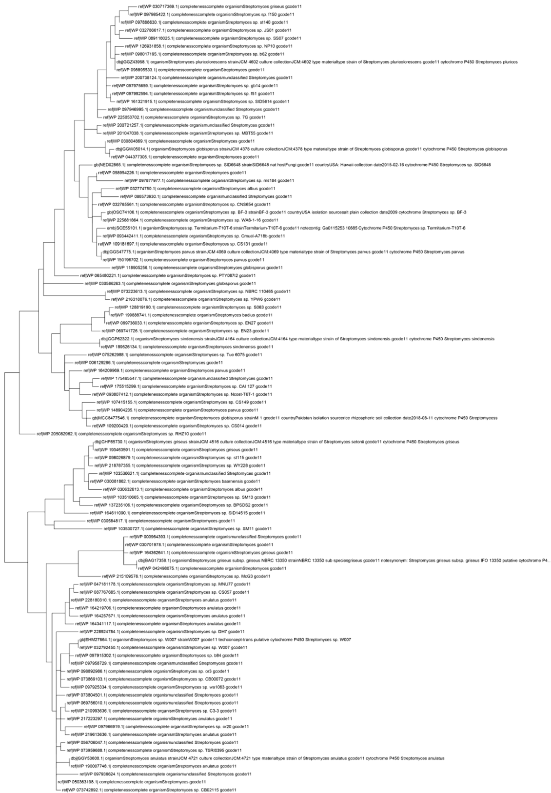
Supplementary Fig. 1. Gene alignment of the P450 enzyme from strain SP6C4 with Streptomyces spp. RAST server (version 2.0) and BVBR, and P450 gene detection using blast N in NCBI DB against Streptomyces species.
